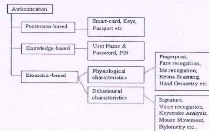
Figure 1. Authentication Methods
